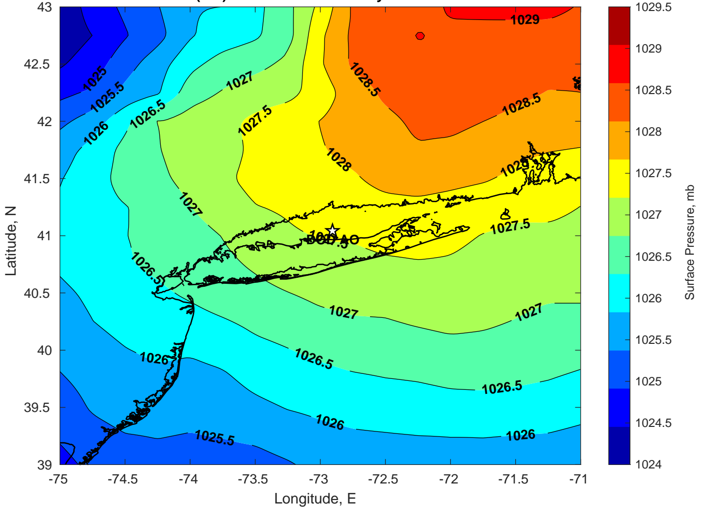
Surface Pressure (mb) for DOD AO at 05-May-2024 06:00:00
